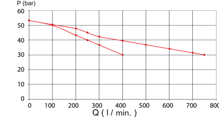
Pressure (Bar) Pump High Pressure Graphic
