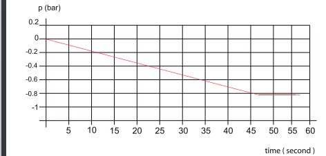
Pressure(Bar) Pump Vacuum Graphic
